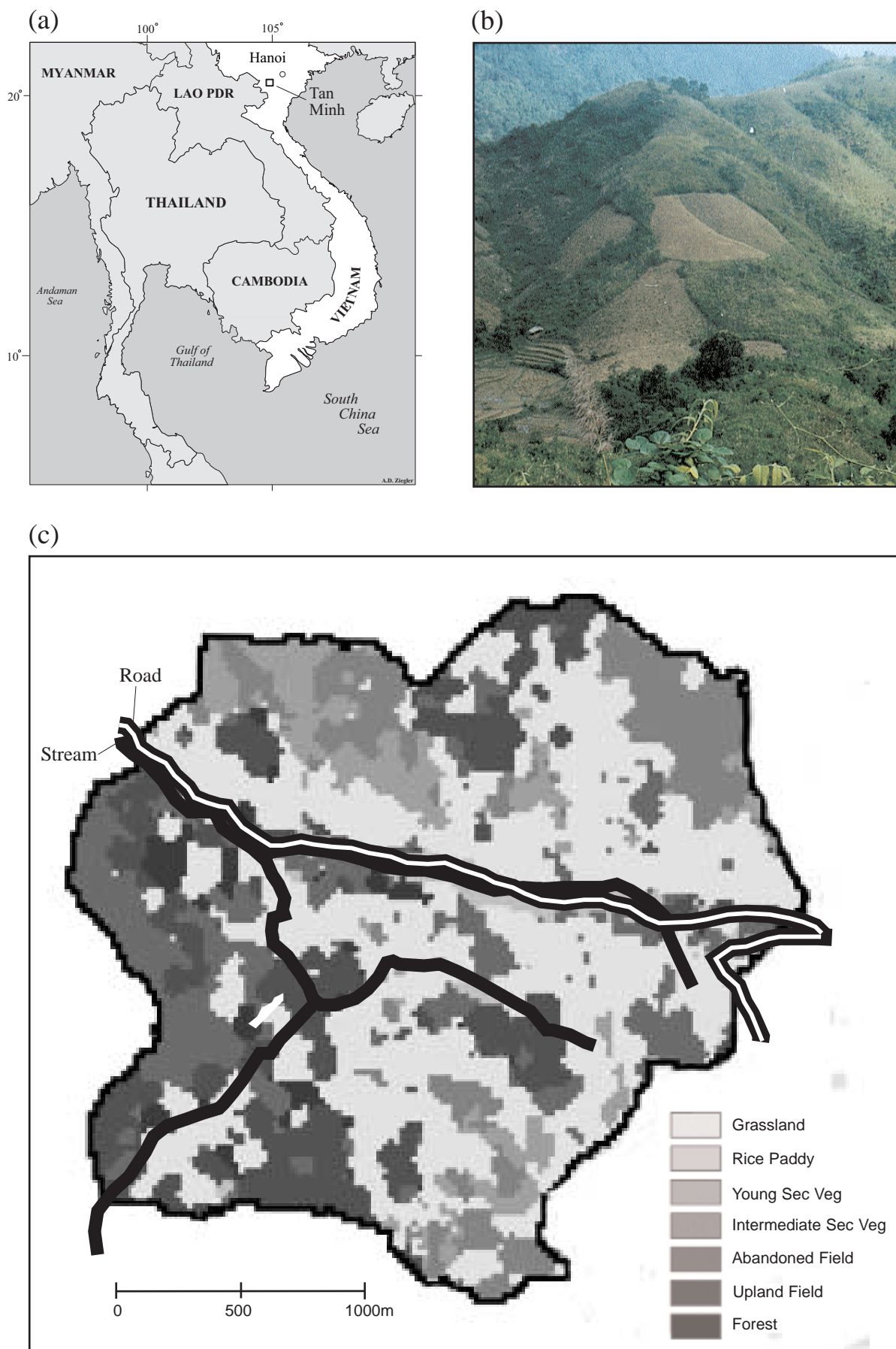
Fig. 1 (a) Tahn Minh, the study area in northern Vietnam; (b) the fragmented landscape in Tahn Minh; (c) land-cover distribution in the 910-ha study watershed.
