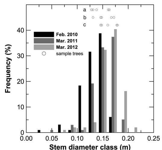
Figure 1. Frequency distribution of stem diameters in the study plot. The values were measured at 1.7-m height above the ground (to avoid the tapping cut) for 98–99 trees in the early part of each year. Trees sampled for sap flow were changed for the three periods (a, January–August 2010; b, August 2010–August 2011; c, August–December 2011).
